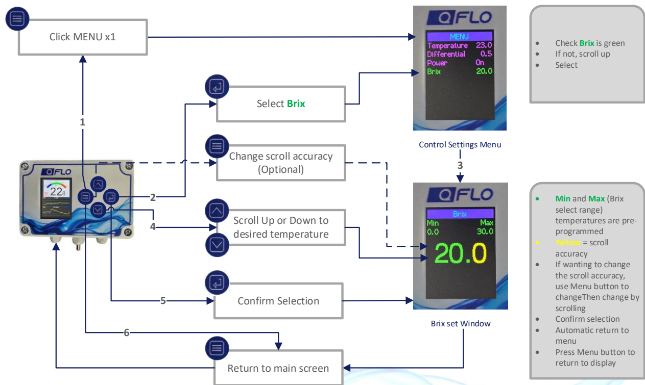
Figure 2: Added Functionality Set-up (Brix Example)
